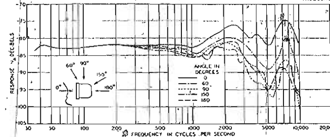
Typical field response of the 618A.
